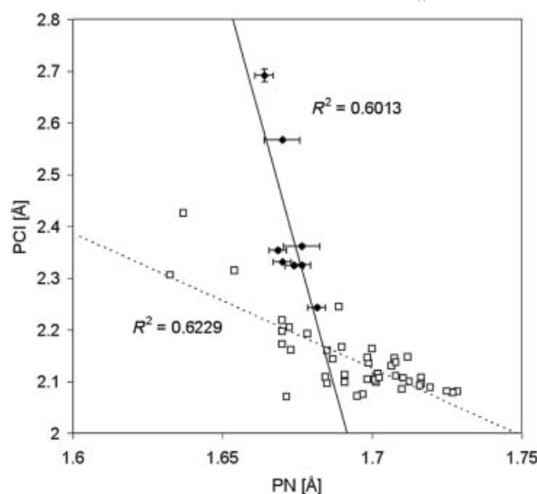
Figure 3. Plot of P–Cl distances [Å] vs. average P–N distances [Å] for 3a–h (diamonds) and for all (R_2N)_2PCl compounds (except 3a,g ) listed in the CSD data base (open squares). The solid and dashed lines represent the result of linear regression analyses. Error bars at the data points for 3a–h denote a range of \pm 3\sigma , where \sigma is the estimated standard deviation. R^2 is the square of the correlation coefficient in the regression analysis.
