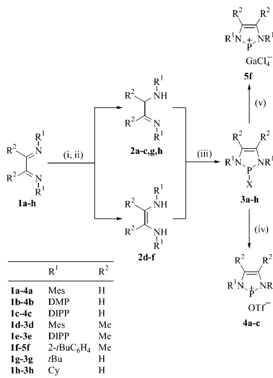
Scheme 2. Synthesis of 2-chloro-1,3,2-diazaphospholenes and 1,3,2-diazaphospholenium salts; (i) 2 Li; (ii) 2 \text{HNEt}_3\text{Cl} , -78^\circ\text{C} ; (iii) \text{PCl}_3 , -78^\circ\text{C} ; (iv) \text{Me}_3\text{SiOTf} , -78^\circ\text{C} – \text{Me}_3\text{SiCl} ; (v) \text{GaCl}_3 . (Mes = 2,4,6- \text{Me}_3\text{C}_6\text{H}_2 , DMP = 2,6- \text{Me}_2\text{C}_6\text{H}_3 , DIPP = 2,6- i\text{Pr}_2\text{C}_6\text{H}_3 ).
