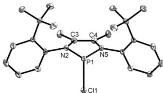
Figure 1. Molecular structure of 3f . Thermal ellipsoids are drawn at the 50% probability level and H atoms have been omitted for clarity.
