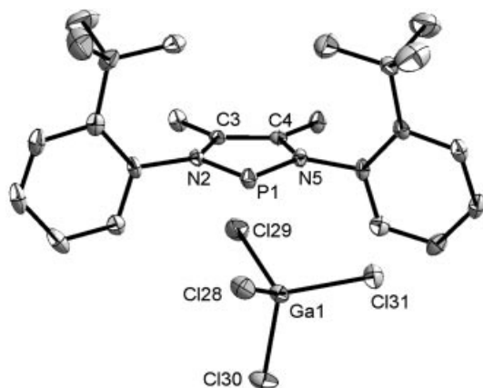
Figure 2. Molecular structure of 5f . Thermal ellipsoids are drawn at the 50% probability level and H atoms have been omitted for clarity.
