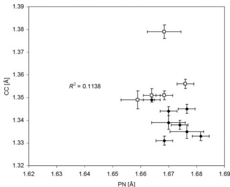
Figure 5. Plot of the average P–N distances [Å] vs. C–C distances [Å] of 3a–h (diamonds) and 4a–c , 5f (open squares). Error bars at each data point denote a range of \pm 3\sigma , where \sigma is the estimated standard deviation.
